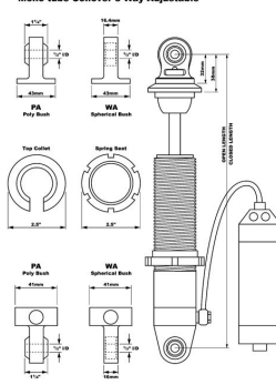
Mono tube Coilover 3 Way Adjustable
