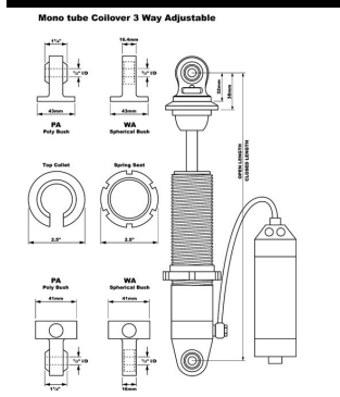
Mono tube Coilover 3 Way Adjustable
