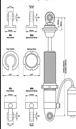
Mono Tube Coilover Single Adjustable
